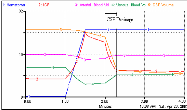
Figure 3: Base simulation run of the ICP dynamic model. The vertical axis show volumes in units of mL and ICP in units of mmHG.
