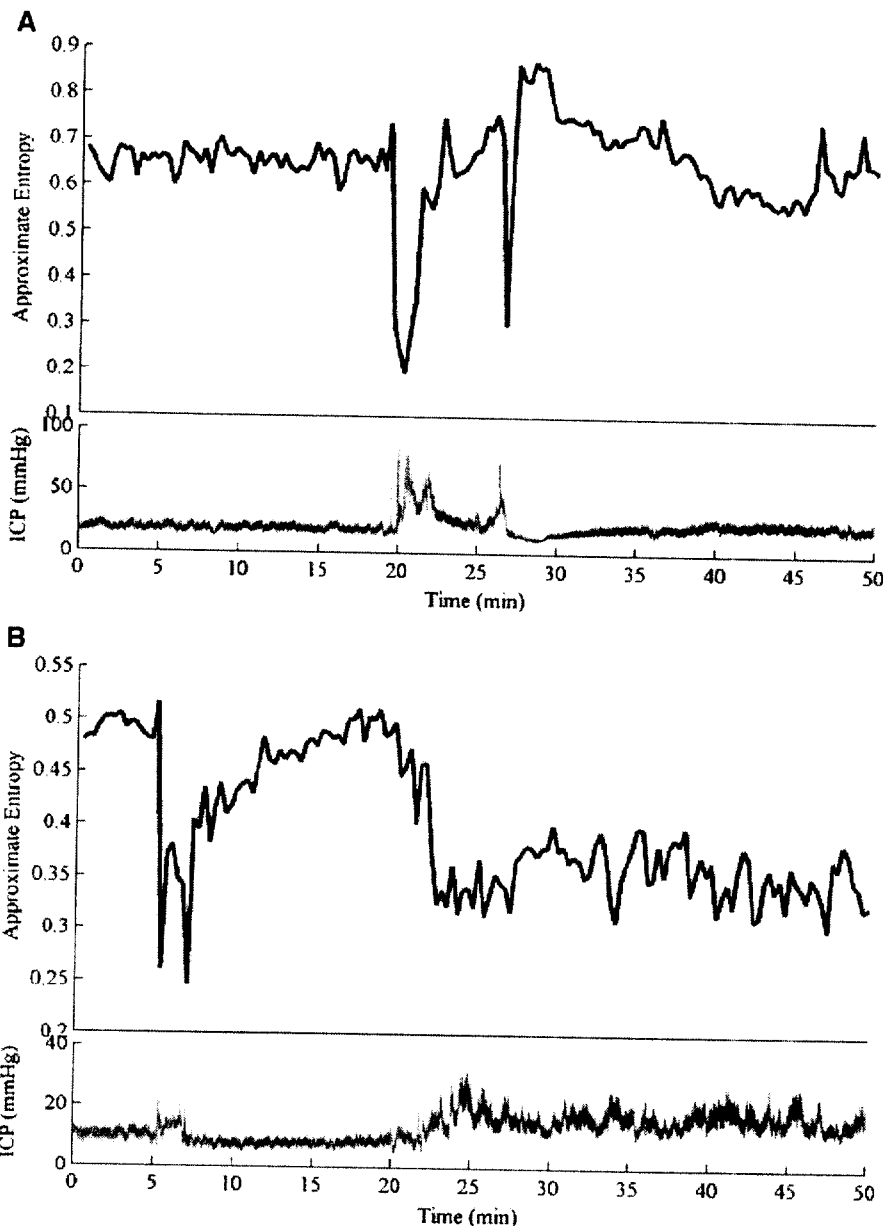
Figure 6. Top , approximate entropy ( ApEn ) vs. intracranial pressure ( ICP ) for patient 1, episode 1. Note decreased ApEn associated with both ICP spikes in pressure >20 mm Hg. Bottom , ApEn vs. ICP for patient 3, episode 1. Note decrease in ApEn during ICP spikes with return to baseline levels during normal ICP .
